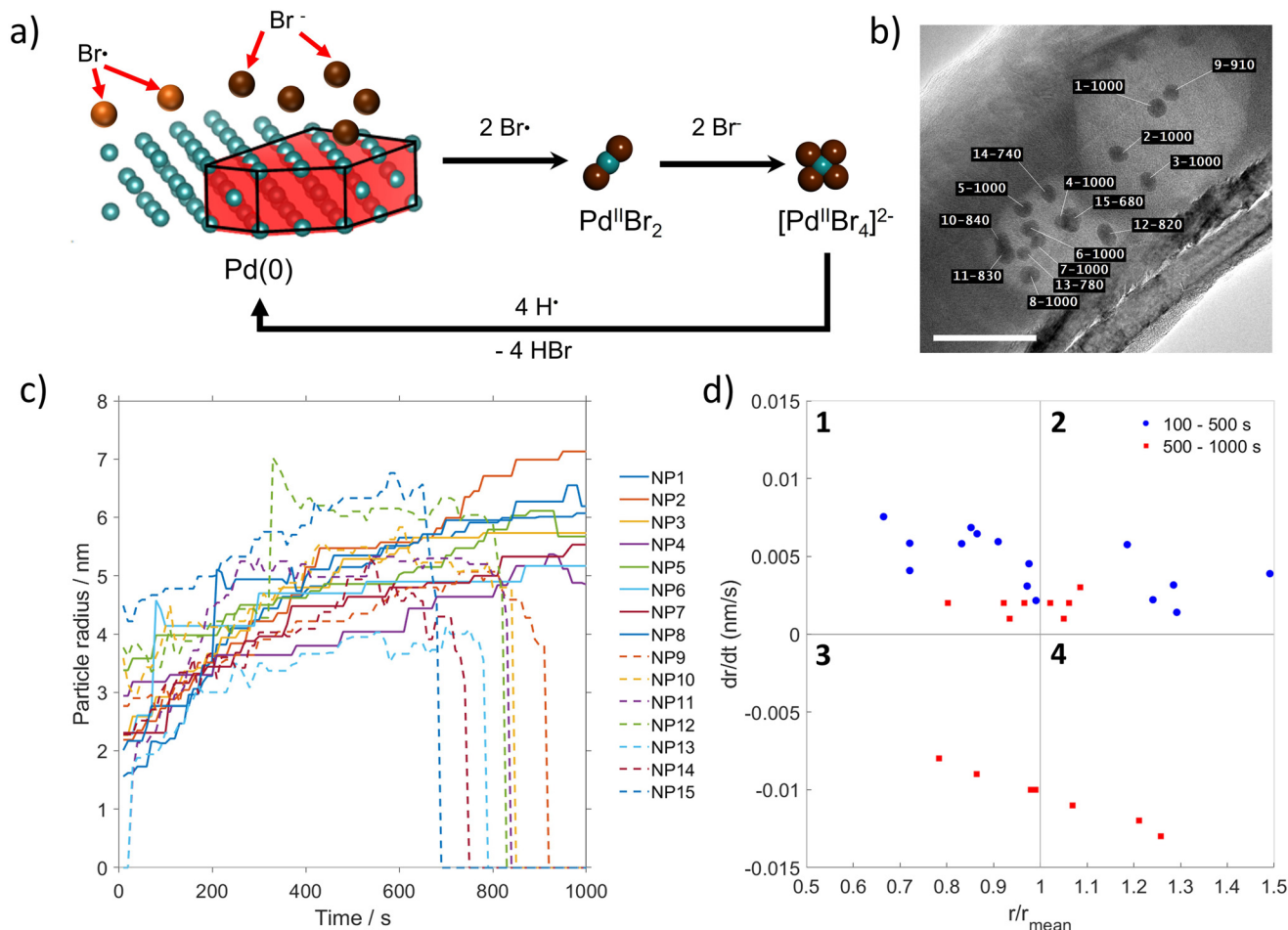
Fig. 6 (a) Oxidation of Pd(0) to Pd(II) by bromine atoms leads to full or partial dissolution of nanoparticles. [\text{PdBr}_4]^{2-} is a soluble form of Pd(II), which can be recycled to grow the next generation of nanoparticles. Reduction of Pd(II) to Pd(0) by hydrogen radicals leads to nanoparticle growth with bromide anions adsorbed on the crystal facets, thus controlling the nanoparticle shape. (b) TEM image highlighting the 15 nanoparticles in IL solution in nanotube present after 500 s of 200 keV electron beam irradiation, the numbers n-m indicate 'number of nanoparticle' – 'time at which the particle was last observed' (a value of m = 1000 indicates that the particle did not undergo dissolution within the 1000 s timeframe). (c) A graph of particle radius plotted against time shows that the Pd NP generally grew at a similar rate for the first 500 s (driven by the reduction of Pd(II) to Pd(0) through DKO) after which some particles dissolved very suddenly (dashed lines; driven by Pd(0) to Pd(II) oxidation by Br - radicals through DVE), and others experienced decreased growth. (d) The rate of growth against the normalised particle size, r/r_{\text{mean}} , allows for the trends to be observed, indicating that the change in particle size was more likely to be due to monomeric addition or migration and coalescence (a minority of cases) over Ostwald ripening. Scale bar is 50 nm.
