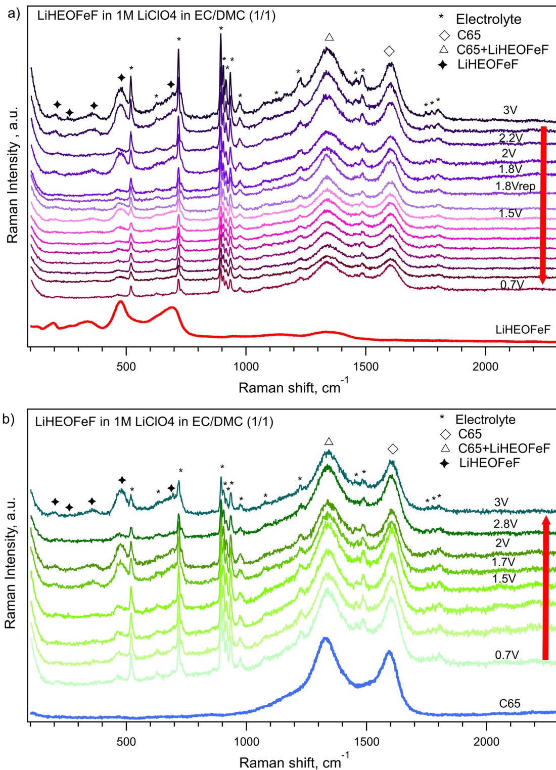
Fig. 8 In situ Raman spectroelectrochemical analysis of coin cells with the LiHFeOFeF cathode and 1M LiClO 4 in ethylene carbonate/dimethyl carbonate (1 : 1 by volume) as the electrolyte solution. (a) Charging of the coin cell from 3 V to 0.7 V vs. Li + /Li. The Raman spectrum of blank LiHFeOFeF is also shown (red line). The label rep stands for repeated measurement at 1.8 V. (b) Discharging of coin cells from 0.7 V to 3 V vs. Li + /Li. The Raman spectrum of the blank C65 additive is also shown (blue line). Spectra are offset, but the intensity scale is identical for all plots.
