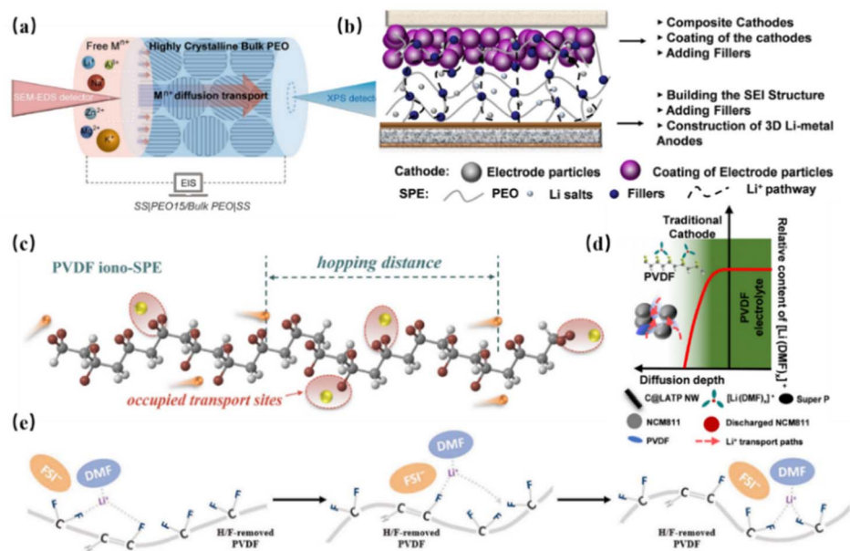
Fig. 3 (a) Schematic of ion diffusion in highly crystalline PEO. 36 (b) Schematic of the PEO-based electrolyte interface and performance enhancement. 43 (c) Schematic representation of \text{Li}^+ transport in the PVDF-based electrolyte. 44 (d) Diffusion of [\text{Li}(\text{DMF})_x]^+ in P-NCM cathodes. 45 (e) Transport mechanism of [\text{Li}(\text{DMF})_x]^+ in residual DMF solvent within the PVDF-based electrolyte. 41
