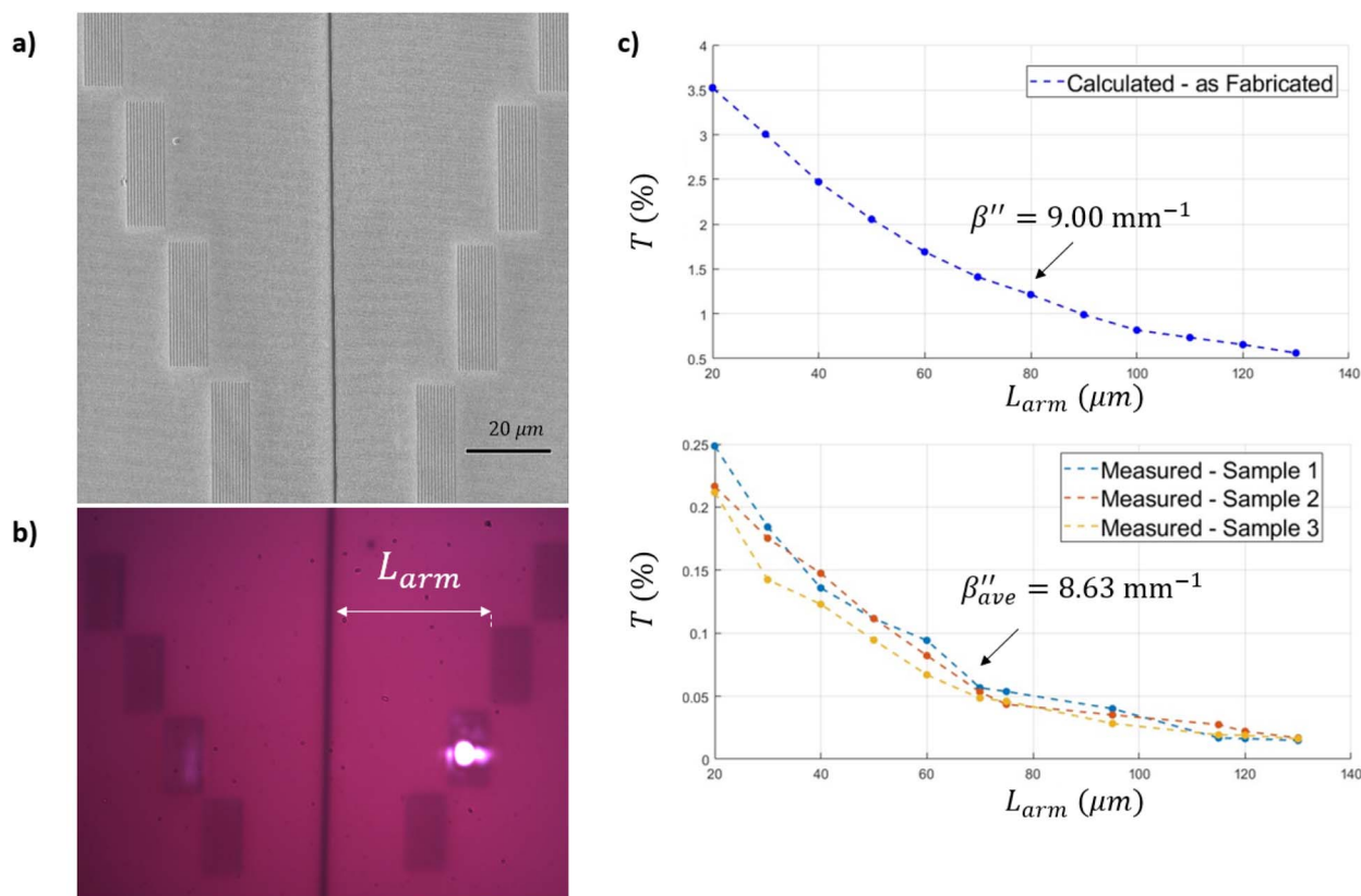
Fig. 6 Cut-back measurements. The distance between the grating and the nanoslit of width w_s = 610 \text{ nm} (arm length) varies from L_{\text{arm}} = 20 to 130 \text{ μm} . (a) SEM image of one of the samples comprised of a linear arrangement of grating couplers along the vertical direction, each grating having a different distance from the nanoslit. (b) Reflected image showing a device under test. A grating coupler is excited with a Gaussian beam of radius w_0 \approx 5 \text{ μm} , aligned near the left edge of the grating. (c), T , for different arm lengths, L_{\text{arm}} . The top panel shows the calculated T as function of L_{\text{arm}} for the simulated case. The attenuation constant can be obtained from an exponential fit of the transmittance curve and is \beta'' = 9.00 \text{ mm}^{-1} , which varies by 6% from the analytical calculation. The bottom panel shows a set of experiments on three samples demonstrating a very similar trend to the calculated cases. The average decay constant obtained experimentally is \beta''_{\text{ave}} = 8.63 \text{ mm}^{-1} , which differs by 1.64% from the analytical calculation.
