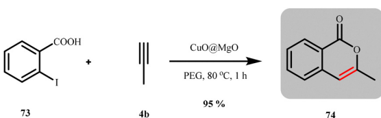
Scheme 35 \text{CuO}@\text{MgO} catalysed synthesis of isocoumarins (Rawat et al. ).
