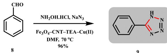
Scheme 4 Catalytic synthesis of heterocyclic derivatives using \text{Fe}_3\text{O}_4 -CNT-TEA-Cu(II) nanoparticles (Akbarzadeh et al. ).
