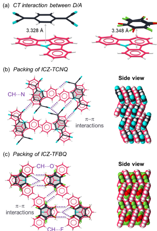
Fig. 2 (a) Interplanar distances between donor and acceptor molecules in ICZ-TCNQ (left) and ICZ-TFBQ (right). Intermolecular π–π (grey) and hydrogen bond (purple) interactions in (b) ICZ-TCNQ cocrystal and (c) ICZ-TFBQ cocrystal with their respective packing.
