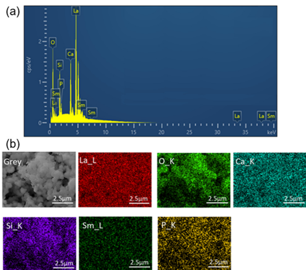
Fig. 5 (a) EDS image and (b) elements mapping analysis of the \text{Ca}_3\text{La}_7(\text{SiO}_4)_5(\text{PO}_4)\text{O}_2:6 \text{ at}\% \text{Sm}^{3+} phosphor.
