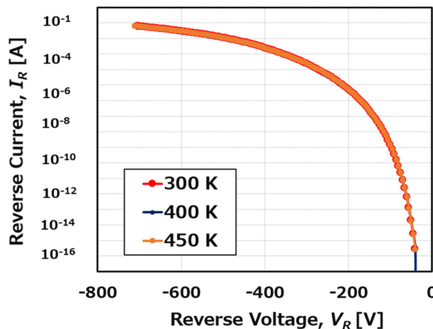
Fig. 6 Simulated temperature-dependent reverse breakdown characteristics of the GaN/ \beta -Ga 2 O 3 p–n diode.
