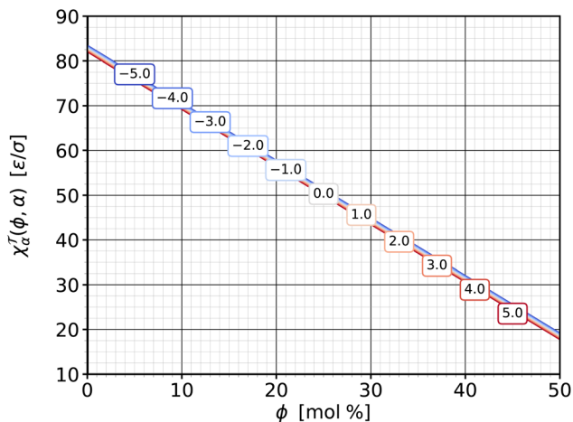
Fig. 9 Susceptibility \chi_{\alpha|\phi}^{\sigma} from eqn (13b) as a function of cholesterol content \phi , parametrized by different values of phospholipid abundance \alpha , as indicated in the boxed labels. The lines almost coincide, with smaller \alpha values having ever so slightly larger susceptibilities.
