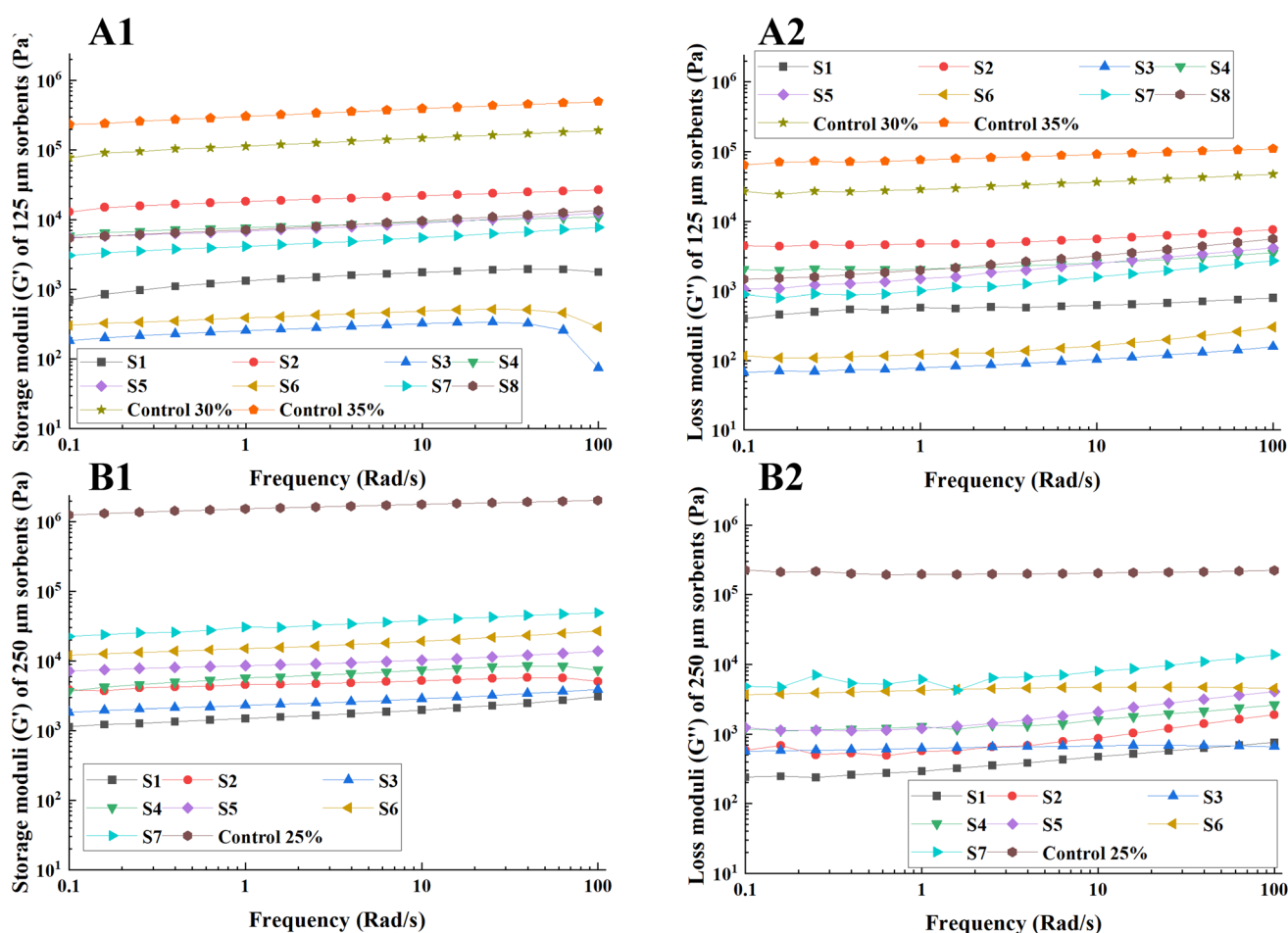
Fig. 5 Frequency sweeping test of sorbents produced using pomelo peel (PP) powders with different particle sizes (125 \mu\text{m} and 250 \mu\text{m} ), oil-to-water ratios (1:3, 1:1, and 3:1), and PP powder concentrations (10–35% w/w); storage moduli (A1) and loss moduli (A2) of 8 sorbent samples (S1–S8) formed from 125 \mu\text{m} PP particles and 2 oil-only sorbents as control samples; storage moduli (B1) and loss moduli (B2) of 7 sorbent samples (S1–S7) formed from 250 \mu\text{m} PP particles and 1 oil-only sorbent as the control sample; details of PP powder concentrations and oil-to-water ratios are presented in Appendix 1.
