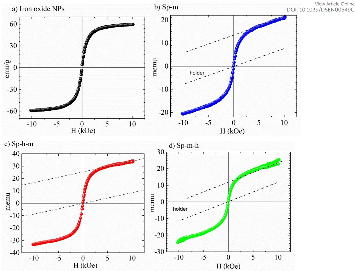
Figure 3. Room temperature magnetic hysteresis loops for all four samples. The hysteresis curve of a) the non-stoichiometric magnetite NPs recorded in powder form, with the Y axis presented in emu/g. For recording the hysteresis curves of the Sp-m, Sp-h-m and Sp-m-h, small pieces of the modified sponges were measured. Their magnetization is provided in memu and the contribution of the sample holders' curve is also presented for clarity (dashed lines). The modified sponges were weighted: b) 1.5 mg Sp-m, c) 2.2 mg Sp-h-m, and d) 2.5 mg Sp-m-h.
