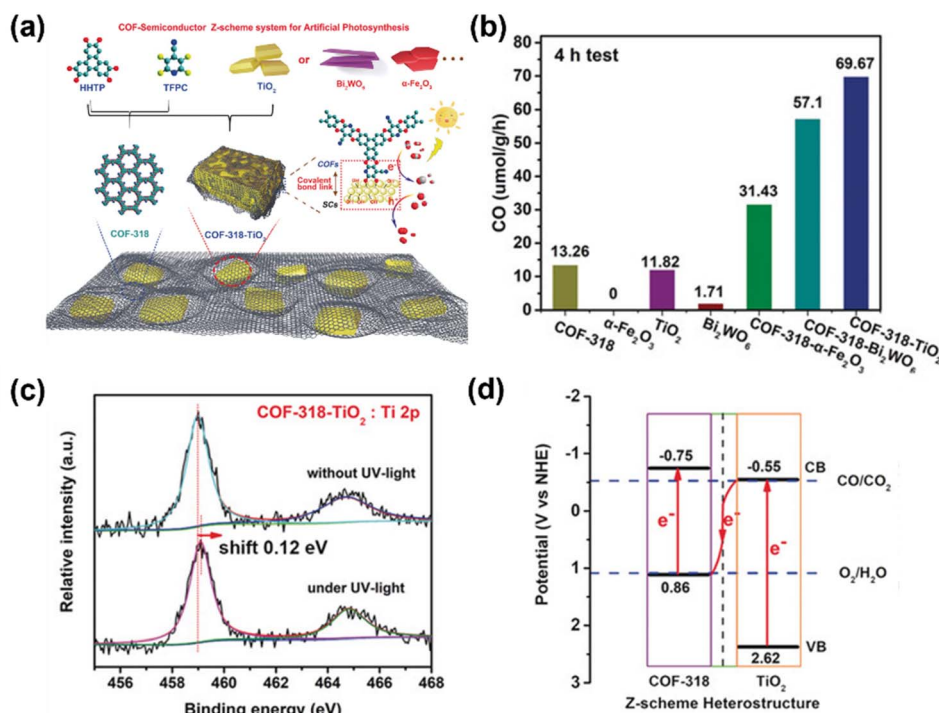
Fig. 12 (a) Schematic illustration of the preparation of COF-318-SCs. (b) Photocatalytic performance of various COF-318-SCs as well as bulk COF-318, TiO 2 , Bi 2 WO 6 , and α-Fe 2 O 3 . (c) High-resolution in situ XPS for Ti 2p of COF-318-TiO 2 in the dark and under 365 nm LED irradiation; (d) schematic illustration of the charge-transfer process under light irradiation with the Z-scheme model. Adapted with permission. 121 Copyright 2020, Wiley-VCH.
