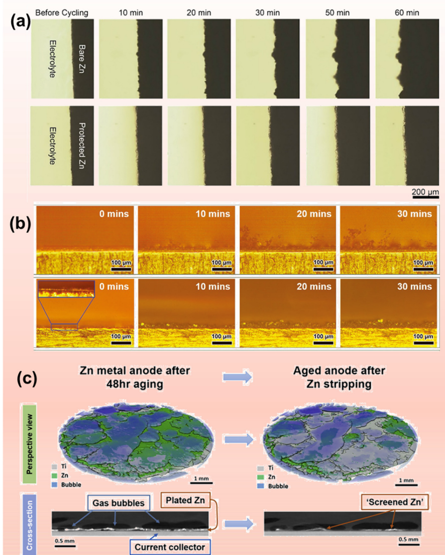
Fig. 24 (a) Operando optical microscopic images of the electrode/electrolyte interface for bare Zn and indium-protected Zn. Reproduced from ref. 120 with permission from Elsevier, copyright 2020. (b) In situ optical images of bare Zn and protected Zn surfaces at a current density of 10 mA cm -2 . Reproduced from ref. 122 with permission from John Wiley & Sons, copyright 2020. (c) In situ CT of Zn anodes undergoing aging. Reproduced from ref. 27 with permission from Cell Press, copyright 2023.
