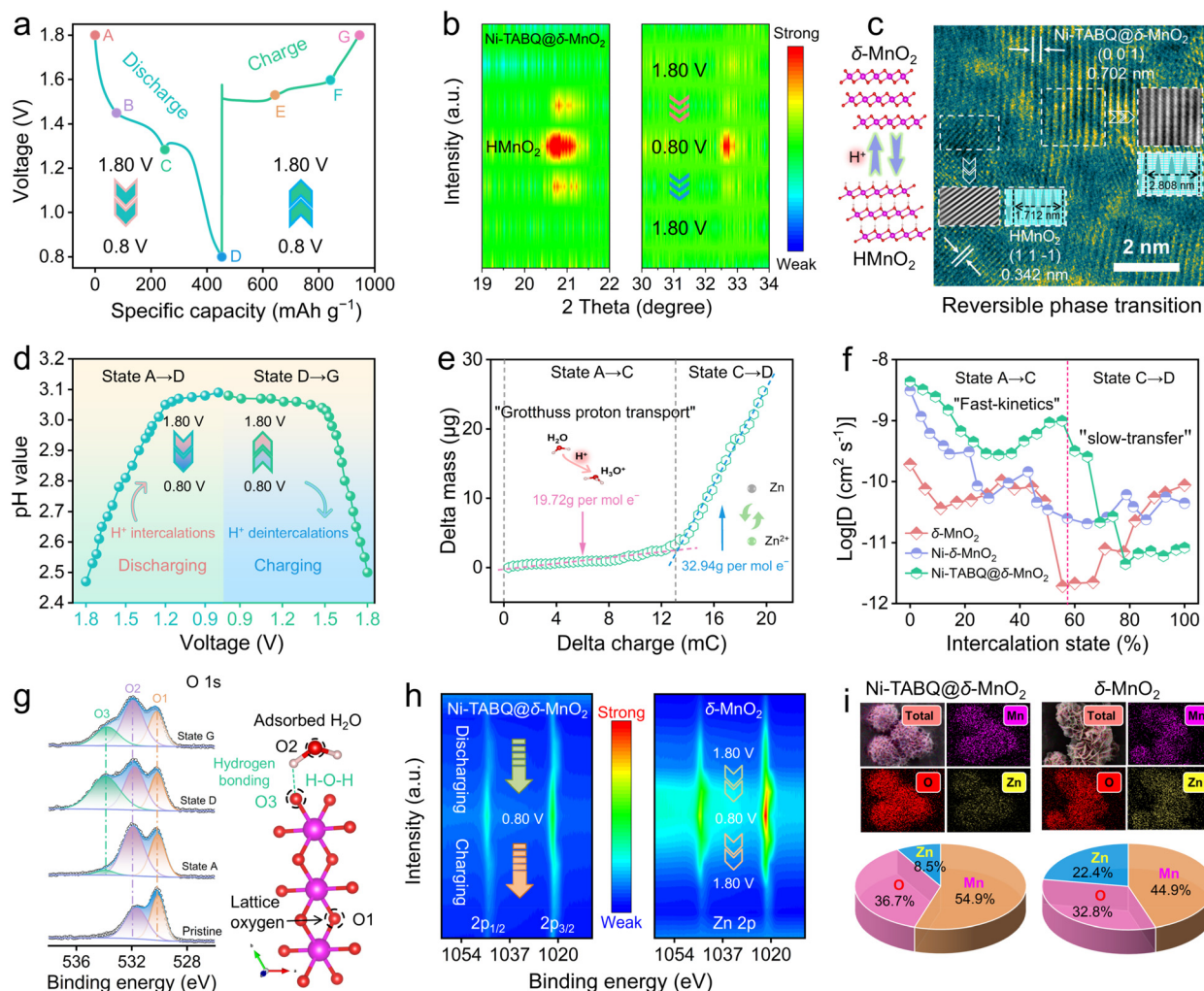
Fig. 4 The Grotthuss proton transfer behavior of the Zn||Ni-TABQ@δ-MnO 2 battery. (a) GCD profiles with selected specific (dis)charge states. (b) Ex situ XRD patterns. (c) A HRTEM image of the Ni-TABQ@δ-MnO 2 cathode in the fully discharged state. (d) In situ pH variations. (e) The electrode mass change versus charge during the discharge (ion-intercalation) process. (f) The ion diffusion coefficient during the discharge process. Ex situ (g) O 1s and (h) Zn 2p XPS spectra. (i) Element maps of Ni-TABQ@δ-MnO 2 and δ-MnO 2 cathodes in the fully discharged state.
