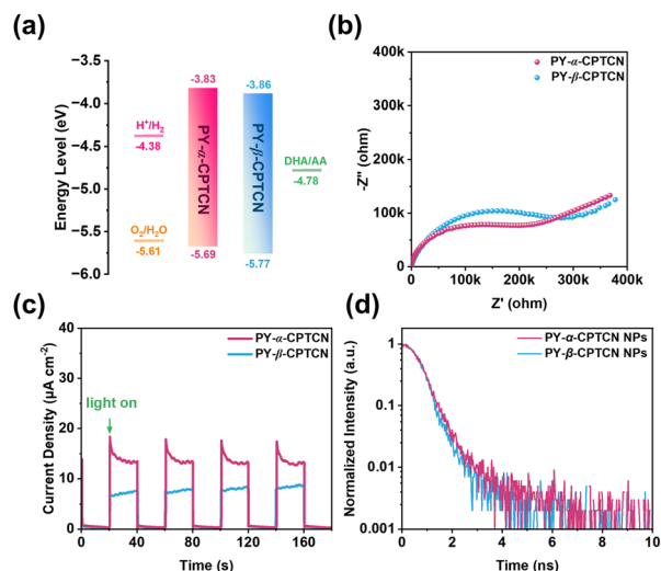
Fig. 3 (a) Energy level alignment of the redox potential of PY-α-CPTCN and PY-β-CPTCN. (b) Electrochemical impedance spectra of these materials. (c) Transient current density vs. time under intermittent light irradiation. (d) Transient PL decay spectra of PY-α-CPTCN and PY-β-CPTCN NPs.
