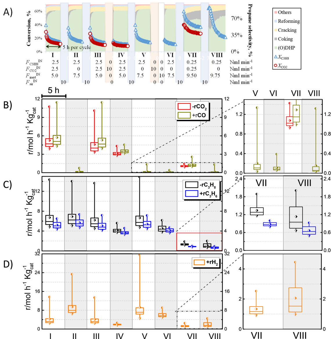
Fig. 8 Variable feed composition applied to 1.3 V/CHA70. A) Propane and CO 2 conversion (left axis) and selectivity (right axis) over 8 cycles (indicated in Roman numerals I–VIII), with a table below detailing the feed composition during each cycle (5 h) and regeneration with F^{IN} representing volumetric flows in NmL\ min^{-1} . B) Box-and-whisker analysis of propane consumption and propylene production. C) 5 Hour box-and-whisker analysis of CO 2 consumption and CO production. (i.e. via ODHP and dry reforming). D) Box-and-whisker analysis of hydrogen production (related to the PDH pathway and deep dehydrogenation). Box and whisker plots excluded the regeneration stages and selected zoom-ins are provided on the right. We loaded 200 mg of V/CHA(70), at a constant T = 600\ ^\circ C , P = 1\ barg . Downstream sampling conducted every 10 minutes.
