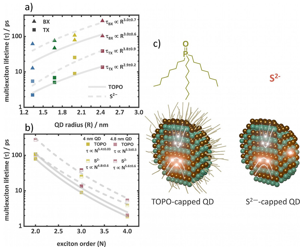
Fig. 4 (a) Dependence of TX and BX lifetimes on the radius of TOPO- and S 2- -capped QDs. (b) Dependence of lifetimes on the exciton order of TOPO- and S 2- -capped 4 nm and 4.8 nm QDs. (c) Illustration of TX, in a TOPO-capped QD with the carrier density concentrated in the CdSe core and in a S 2- -capped QD with a trapped hole on the surface site.
