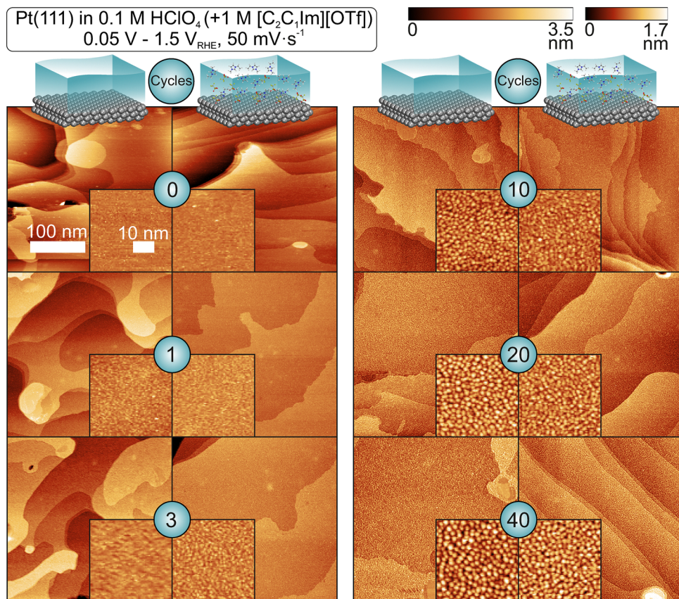
Fig. 4 EC-STM images ( U_{\text{bias}} 0.4 \text{ V} , I_t 0.2\text{--}1 \text{ nA} ) before and after the initial oxidation–reduction cycles ( 0.05\text{--}1.5 V_{\text{RHE}} , 50 \text{ mV s}^{-1} ) in the absence (left) and presence (right) of 1 \text{ M } [\text{C}_2\text{C}_1\text{Im}][\text{OTf}] . Supporting electrolyte was 0.1 \text{ M HClO}_4 .
