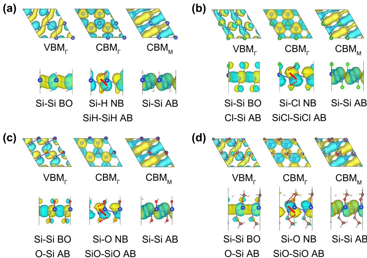
Fig. 3 The top and side views of the VBM \Gamma , CBM \Gamma , and CBM M orbitals of (a) SiH, (b) SiCl, (c) SiOH, and (d) SiOCH 3 . The characters of the orbitals with respect to certain pairs of atoms are specified: BO = bonding orbital, NB = nonbonding, and AB = antibonding.
