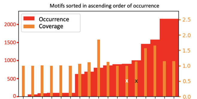
Fig. 9 Distribution of the number of occurrences and coverage rate between motifs of size 3 that contain at least one hydrogen bond and one oxygen atom of the surface, that are being recognized over the 100 conformations extracted from the (110)-quartz/liquid water interface trajectory. The black and white crosses respectively report the ranking of motif M1 and M2 .
