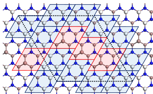
Fig. 11 Top view of the stable ( 6 \times 6 ) surface structure by the arrangements of the hydrogen-covered surface (blue tiles) and the Ga adatom surface (red tiles), discovered by the Bayesian optimization. Brown, blue and white atoms correspond to Ga, N and H, respectively. Black dashed tile indicates a ( 6 \times 6 ) area. Reproduced from ref. 112 with permission from American Institute of Physics, copyright 2022.
