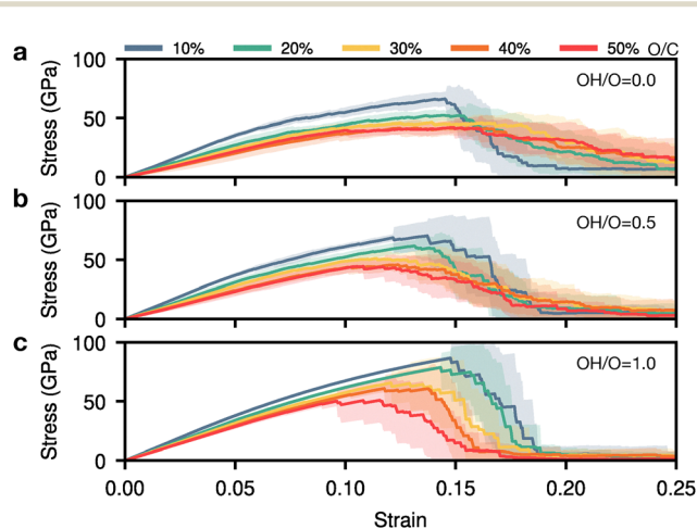
Fig. 2 Mechanical behaviour of GO and its dependence on the oxygen content. We show stress-strain curves for 20 GO sheets of ~200 atoms each, at varying O/C ratio (indicated by colour-coding). The shaded areas indicate one standard deviation. We characterise sheets that have been functionalised: (a) fully with epoxide groups; (b) with half epoxide, half hydroxyl groups; and (c) fully with hydroxyl groups.
