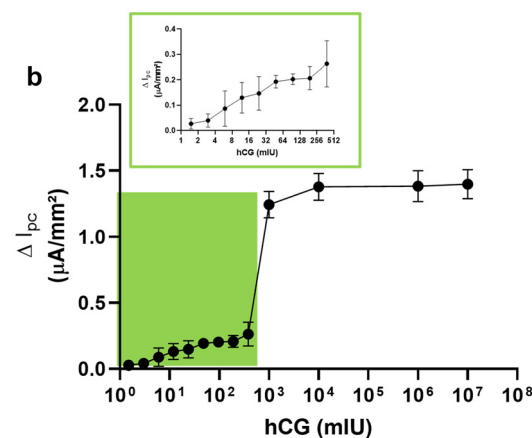
Fig. 3 (a) Current change (measured using cyclic voltammetry) of the E-layer-entrapped hCG nanoMIPs following rebinding of hCG at 24–10000 mIU. The inset shows the increase in peak cathodic current with increasing hCG levels within the lower concentration range. (b) hCG levels in mIU plotted against the peak cathodic current change ( \Delta I_{pc} ). The inset shows the concentration-dependent response range (1.5–384 mIU). As the hCG concentration increases, the \Delta I_{pc} value increases proportionately until saturation of the nanoMIP binding sites is reached.
