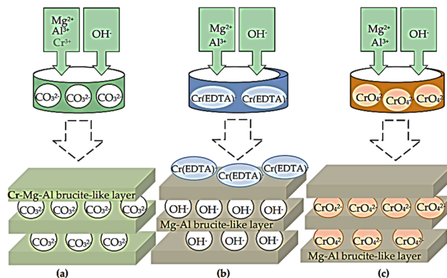
Scheme 3 Synthetic methods for producing chromium catalyst LDH precursors.
