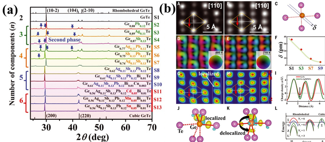
Fig. 18 (a) XRD patterns of GeTe based high entropy materials at room temperature. Secondary phases as indicated by the blue arrow were seen for samples with less components; (b) (A)–(L) images depict the delocalization of the electrons and off-centering of Ge in the high entropy GeTe alloys. Reproduced and adapted from ref. 135. Copyright © 2022, The American Association for the Advancement of Science.
