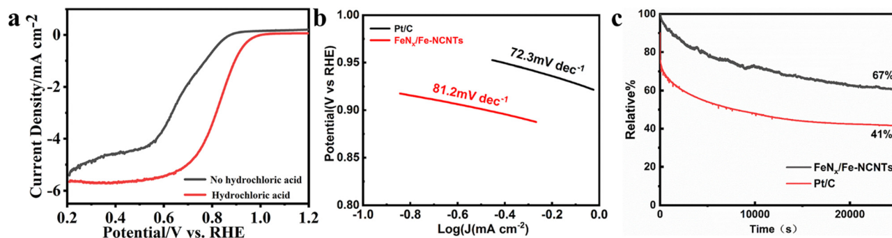
Fig. 6 (a) LSV curves of FeN x /Fe-NCNTs in the presence or absence of hydrochloric acid (1600 rpm); (b) Tafel slopes of FeN x /Fe-NCNTs and Pt/C catalysts; (c) chronoamperometry of FeN x /Fe-NCNTs and Pt/C at 0.6 V (vs. RHE).
