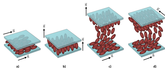
Fig. 6 Various orientations of mesogens in LCEs: (a) planar, where mesogens align parallel to the alignment surfaces, (b) homeotropic, where mesogens align perpendicular to the alignment surfaces, (c) twisted nematic, with a mixture of mesogens aligned both perpendicular and parallel to the alignment surfaces, and (d) splay, where mesogens align parallel to the alignment surfaces but with a 90-degree rotation.
