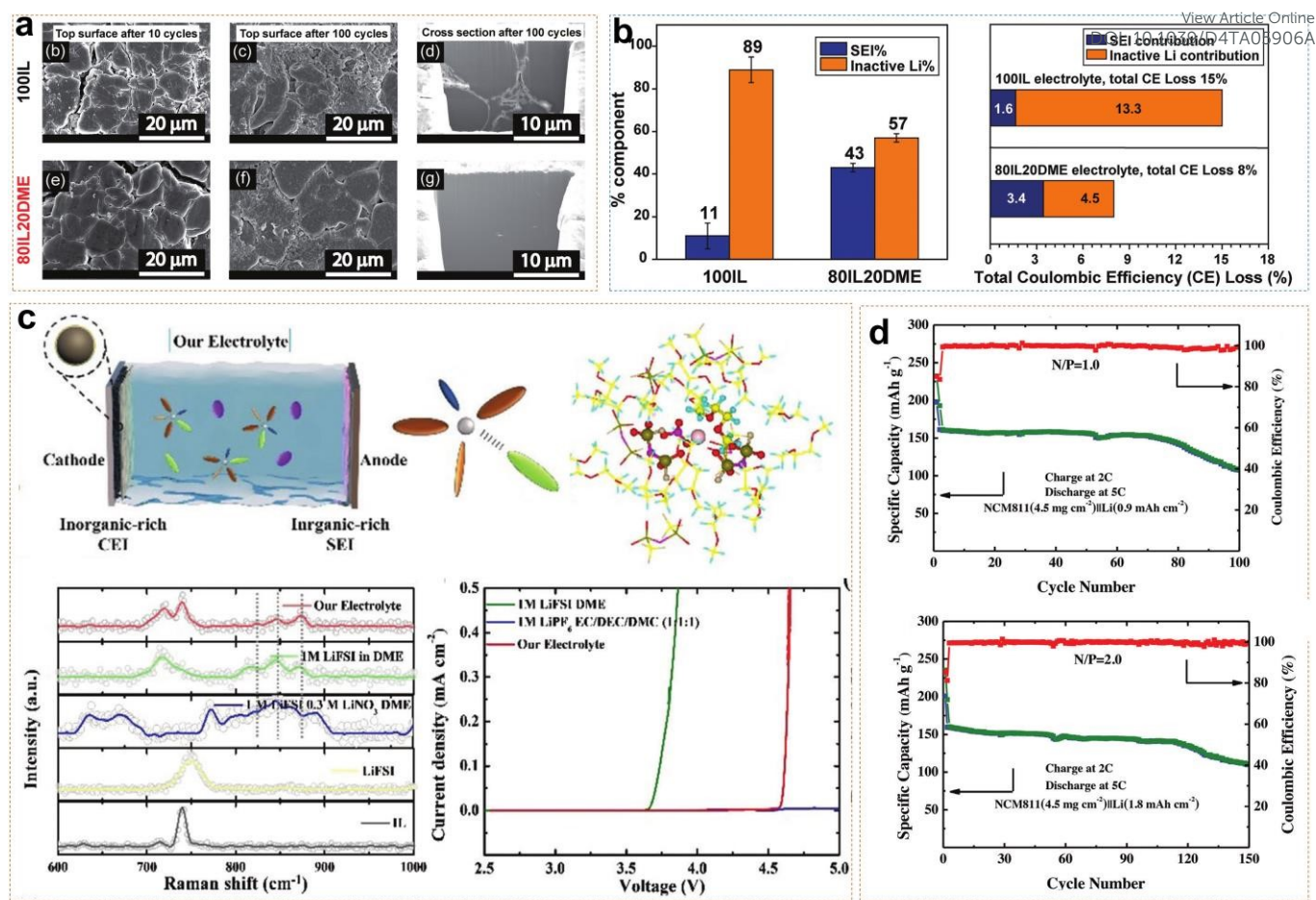
Fig. 6 (a) Morphology of top surface and cross-section by Cryo-FIB in 100IL and 80IL20DME electrolyte. (b) Quantitative analysis of \text{Li}^0_{\text{inactive}} and \text{Li}^+_{\text{SEI}} by TGC quantification method. Reprinted from ref. 45 with permission. Copyright 2022, The Royal Society of Chemistry. (c) Schematically illustration of Li/NCM811 full cells in IL-based electrolytes; Raman spectra, and liner sweep voltammetry curves. (d) Cycling performance of Li/NCM811 full cell under N/P ratio of 2 and 1. Reprinted from ref. 46 with permission. Copyright 2023, Wiley.
