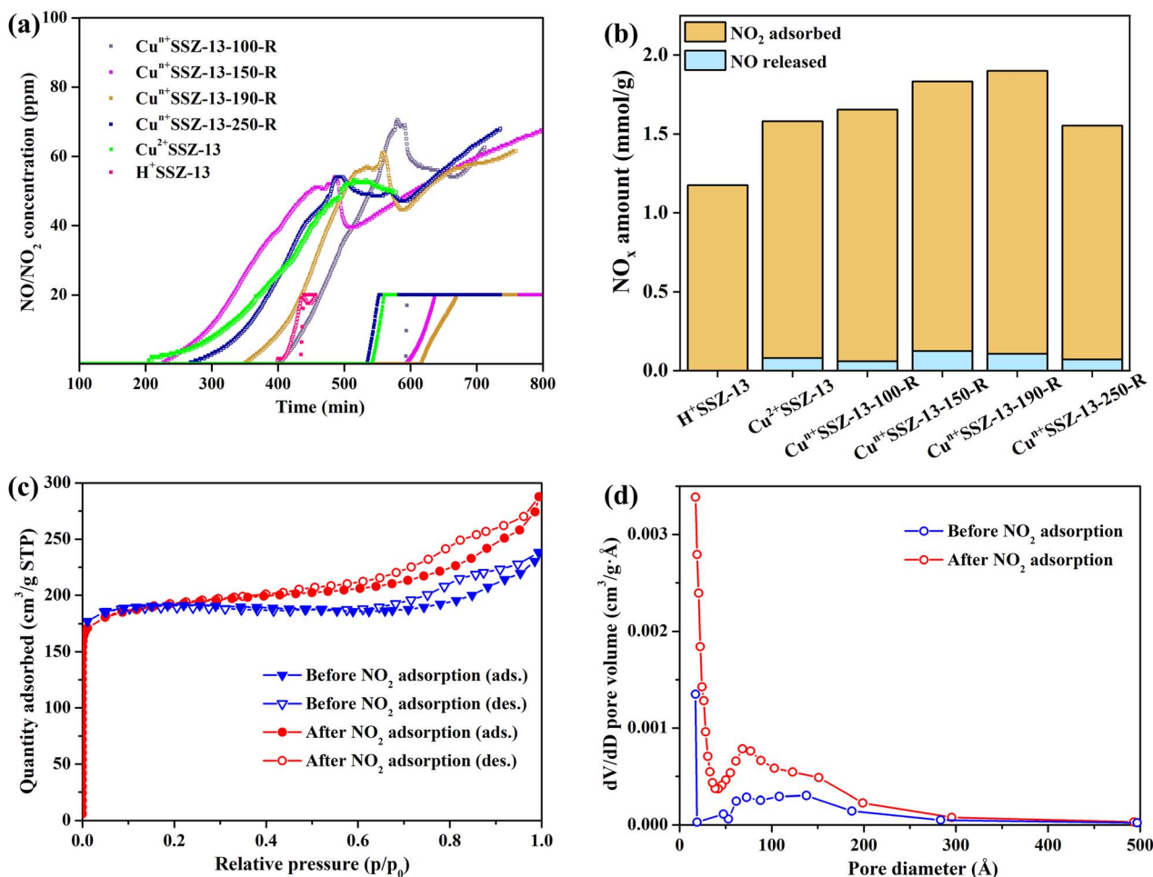
Fig. 4 (a) \text{NO}_2 (1000 ppm) dynamic column adsorption at room temperature on \text{H}^+ SSZ-13, \text{Cu}^{2+} SSZ-13 and \text{Cu}^{n+} SSZ-13 samples with thermal activation. The hollow ( \square ) and solid ( \blacksquare ) dots represent the concentration of NO and \text{NO}_2 , respectively. (b) The corresponding \text{NO}_2 adsorption capacity and NO released amount. (c) \text{N}_2 adsorption–desorption isotherms ( -196^\circ\text{C} ) and (d) pore size distributions of \text{Cu}^{n+} SSZ-13-190-R before and after \text{NO}_2 (1000 ppm) dynamic column adsorption.
