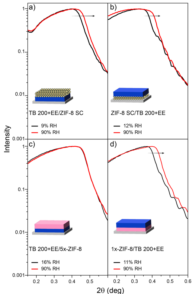
Fig. 3 XRR experiments for dry and vapour-saturated atmospheres for samples: (a) TB 200+EE/ZIF-8 SC, (b) ZIF-8 SC/TB 200+EE, (c) TB 200+EE/5x-ZIF-8 and (d) 1x-ZIF-8/TB 200+EE.
