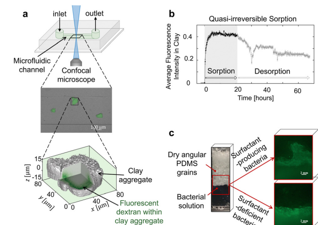
Fig. 16 (a) Microfluidic experiments showing the sorption and desorption of a fluorescently-labeled organic matter in clay. The propagation of the green fluorescent dextran (sugar) into the clay (gray color) was visualized in 3-dimensional space over time. 357 (b) The quasi-irreversible sorption of a large molecular weight (>3 kDa) dextran with a clay aggregate. 357 (c) A surfactant-producing bacterium, Pseudomonas aeruginosa (labeled with green fluorescence), spreads into a synthetic soil placed on top of the bacterial solution, while a surfactant-deficient mutant does not. 358 The scale bars in (a) and (c) are 100 \mu\text{m} and 2 mm, respectively.
