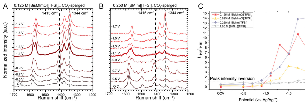
Fig. 5 In situ SERS spectra of 0.125 M [BisMimO][TFSI] 2 (A) and 0.250 M [BMim][TFSI] (B) under \text{CO}_2 -sparged conditions. The potential at which the 1344\text{ cm}^{-1} peak intensity surpasses the 1415\text{ cm}^{-1} peak is bolded. The relative intensities of the 1344 and 1415\text{ cm}^{-1} peaks are used to determine the extent of imidazolium reorientation (C). The normalized peak intensity of the 1344\text{ cm}^{-1} peak surpasses that of the 1415\text{ cm}^{-1} peak at -1.1\text{ V vs. Ag/Ag}^+ for both samples. Comparing the ratios of the peak intensities of the 1344 to 1415\text{ cm}^{-1} peaks, we find that the 1.65 M [BMim][TFSI] inversion potential is more negative than the other ionic liquid concentrations. The inversion potential for the 0.825 M [BisMimO][TFSI] 2 remains similar to the lower concentration electrolytes, which suggests that the covalent link provides a “pre-structuring” effect between the two imidazoliums of the [BisMimO] + cation.
