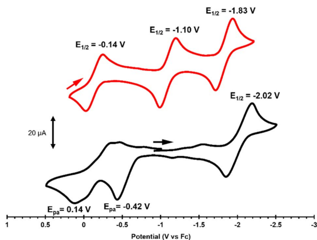
Fig. 3 Cyclic voltammograms of 1 (bottom, black) and 2 (top, red) in 0.1 M [ t Bu 4 N][PF 6 ] solution (scan rate = 100 mV s -1 ). All potentials are referenced to Fc/Fc + .
