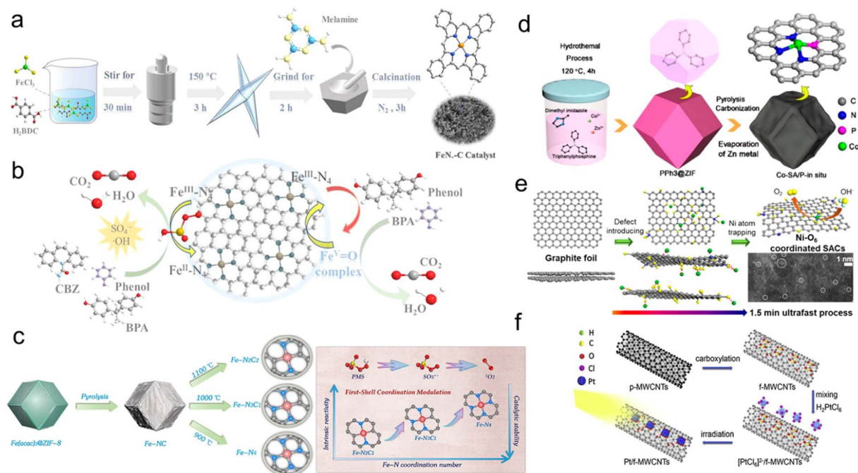
Fig. 6 (a) The preparation of Fe x N x -C catalysts (Fe SACs); (b) the proposed mechanism of Fe x N x -C/PMS system; 86 Copyright 2021 American Chemical Society. (c) The synthesis strategy of Fe x N x catalysts based on pyrolysis temperature and the relationship between Fe–N coordination number and the intrinsic reactivity; 150 Copyright © 2023 American Chemical Society. (d) The fabrication process of Co-SA/P catalysts; 153 Copyright © 2020 American Chemical Society. (e) Schematic of the synthesis process for Ni SACs; 161 Copyright © 2020 American Chemical Society. (f) The preparation strategy of Pt/f-MWCNTs; 162 figures have been adapted from ref. 86, 150, 153, 161 and 162 with permissions from the American Chemical Society, Copyright 2022, American Chemical Society, Copyright 2023, American Chemical Society, Copyright 2020, American Chemical Society, Copyright 2020 and Elsevier B.V. Copyright 2019, respectively.
