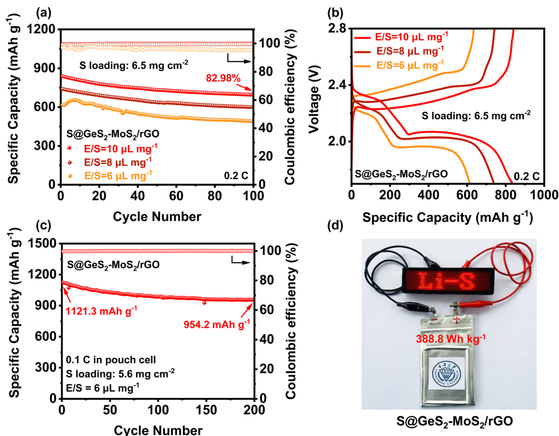
Fig. 6 (a) Cycling performances of the \text{S@GeS}_2\text{-MoS}_2/\text{rGO} cathode with different E/S ratios at 0.2C. The \text{S@GeS}_2\text{-MoS}_2/\text{rGO} cathode obtains stable cycling and high capacity retention after 100 cycles, showing excellent sulfur utilization at low electrolyte usage. (b) Galvanostatic discharge/charge profiles of the \text{S@GeS}_2\text{-MoS}_2/\text{rGO} electrode with different E/S ratios at 0.2C. (c) Cycling stability of a pouch cell with the \text{S@GeS}_2\text{-MoS}_2/\text{rGO} electrodes at 0.1C. The \text{S@GeS}_2\text{-MoS}_2/\text{rGO} cathode maintains a high and stable capacity, suggesting potential electrochemical performance in practical applications. (d) Optical photograph of a pouch cell based on \text{S@GeS}_2\text{-MoS}_2/\text{rGO} electrodes charging a "Li-S" shaped LED.
