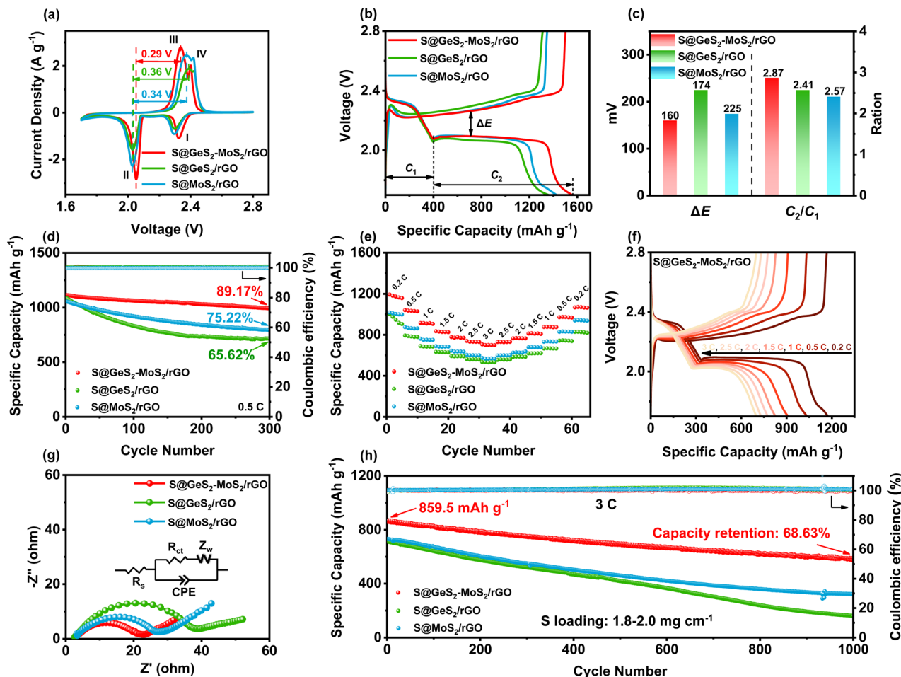
Fig. 5 (a) CV curves of different electrodes at a scan rate of 0.1 \text{ mV s}^{-1} within 1.7–2.8 V. The S@GeS 2 -MoS 2 /rGO cathode shows the lowest potential, indicating enhanced redox kinetics. (b) Galvanostatic discharge/charge profiles of different electrodes at a 0.1C current rate. (c) \Delta E and C_2/C_1 values of galvanostatic discharge/charge profiles. The S@GeS 2 -MoS 2 /rGO cathode exhibits the lowest polarization potential and highest C_2/C_1 value, demonstrating its excellent electrocatalytic activity. (d) Cycling life of different electrodes at 0.5C over 300 cycles. (e) Rate performance of different electrodes with various current densities. The S@GeS 2 -MoS 2 /rGO electrode displays the highest capacity retention and rate capacities. (f) Galvanostatic discharge/charge profiles of S@GeS 2 -MoS 2 /rGO at various current densities. (g) EIS spectra of different cathodes after 100 cycles. GeS 2 -MoS 2 /rGO exhibits a minimal R_{ct} value, which is attributed to the excellent electrical conductivity of the heterostructure. (h) Cycling stability of different electrodes at 3C over 1000 cycles. The S@GeS 2 -MoS 2 /rGO electrode shows a high discharge capacity and stable cycling performance, indicating that LiPS shuttling during cycling is effectively suppressed.
