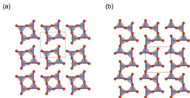
Fig. 10 The outer \text{SbO}_2 sublayer of a triple fluorite block in (a) \text{Sb}_2\text{-YO}_4\text{Cl} and (b) \text{Sb}_2\text{MO}_4\text{Br} ( M = \text{Y}, \text{Eu-Tb} ). \text{Bi}_2\text{MO}_4\text{Cl} possesses 1D chains of corner-sharing \text{BiO}_3 (see Fig. 9 for comparison), while in \text{Sb}_2\text{YO}_4\text{Cl} , 0D \text{Sb}_4\text{O}_8 (0D) rings are formed. Purple and red balls represent Sb and O, respectively.
