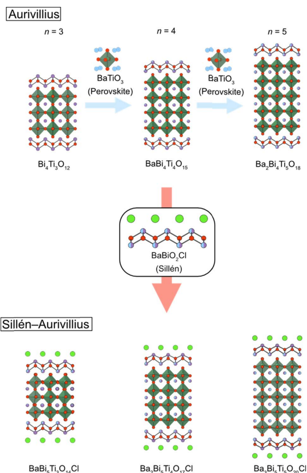
Fig. 15 An illustration of the bricklaying synthesis for multi-layered Sillén–Aurivillius phases \text{BaBi}_5\text{Ti}_5\text{O}_{20}\text{Cl} ( n = 3 ), \text{Ba}_2\text{Bi}_5\text{Ti}_5\text{O}_{17}\text{Cl} ( n = 4 ) and \text{Ba}_3\text{Bi}_5\text{Ti}_5\text{O}_{20}\text{Cl} ( n = 5 ). 38
