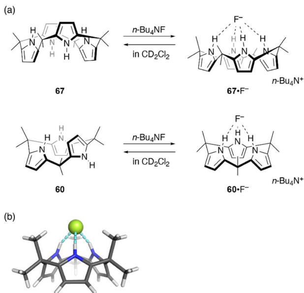
Fig. 11 (a) Fluoride binding to calix[4]pyrrole 67 and calix[3]pyrrole 60 . (b) Crystal structure of 60 · \text{F}^- .
