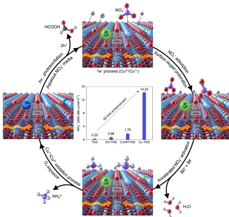
Fig. 9 \text{NO}_3^- -to- \text{NH}_3 reaction mechanism on Cu-TNSs. TiO 2 with isolated Cu 2+ atomic sites (blue) and defects generates photoexcited electrons and holes under light irradiation. 118
