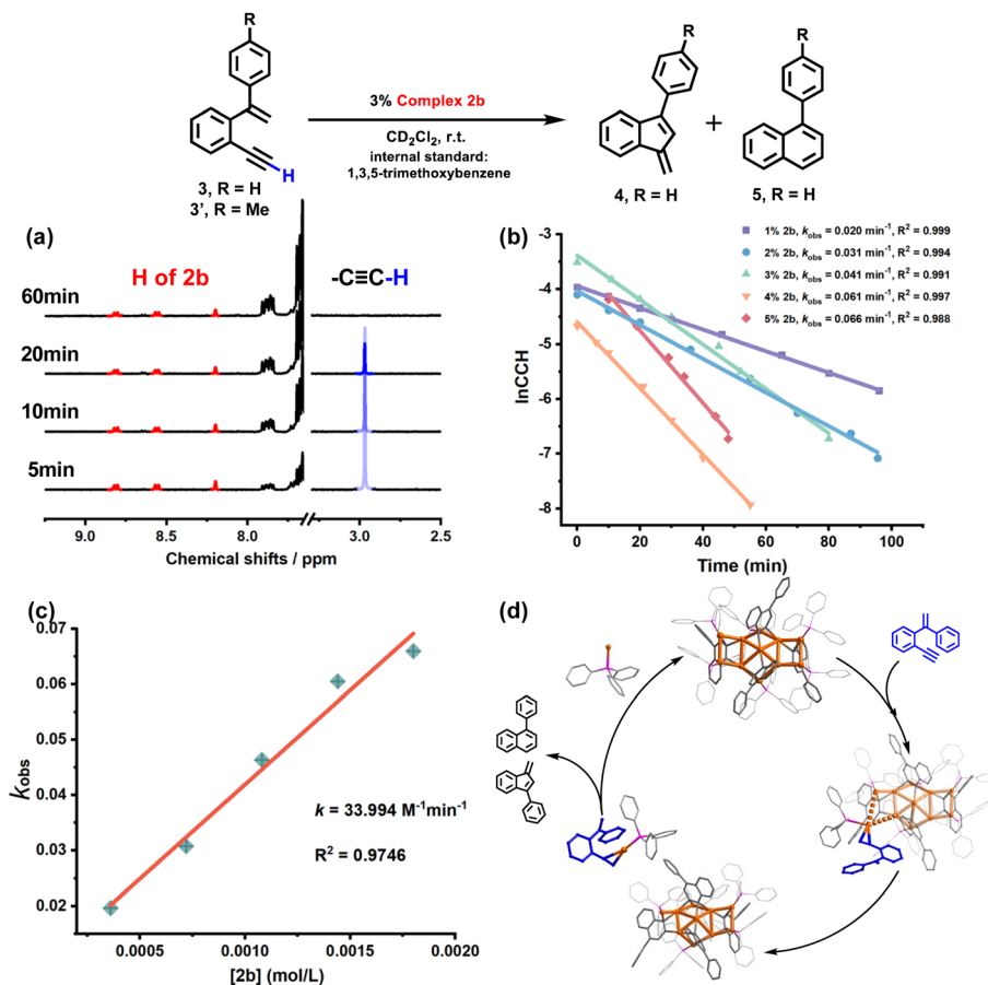
Fig. 3 (a) 1 H NMR monitoring of the 2b -catalyzed cyclization reaction. Red and blue lines represent the proton NMR peaks of 2b and the alkyne substrate, respectively. (b) Pseudo-first-order kinetic curves dependent on the concentration of 2b . (c) Kinetic curves of 2b dependent on the catalyst concentration. (d) Proposed mechanism for the cyclization reaction catalyzed by 2b .
