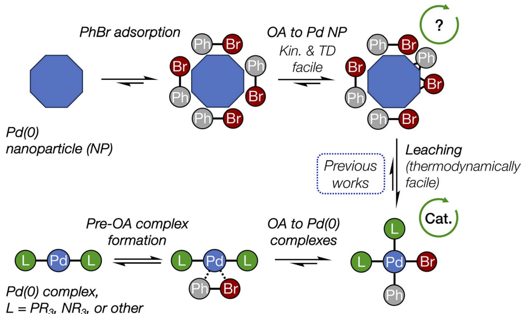
Fig. 4 The interplay of oxidative addition in catalyst interconversions in the course of (cross-)couplings with \text{Pd}(0) nanoparticles and molecular complexes. See Fig. 2 for more detailed structures and Fig. 3 for reaction (activation) free energies. The arrowed circles represent (possible) participation in the catalytic cycle (see text for discussion).
