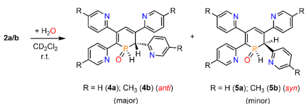
Scheme 2 Reaction of 2a/b with \text{H}_2\text{O} under formation of diastereomers 4a/b and 5a/b .
