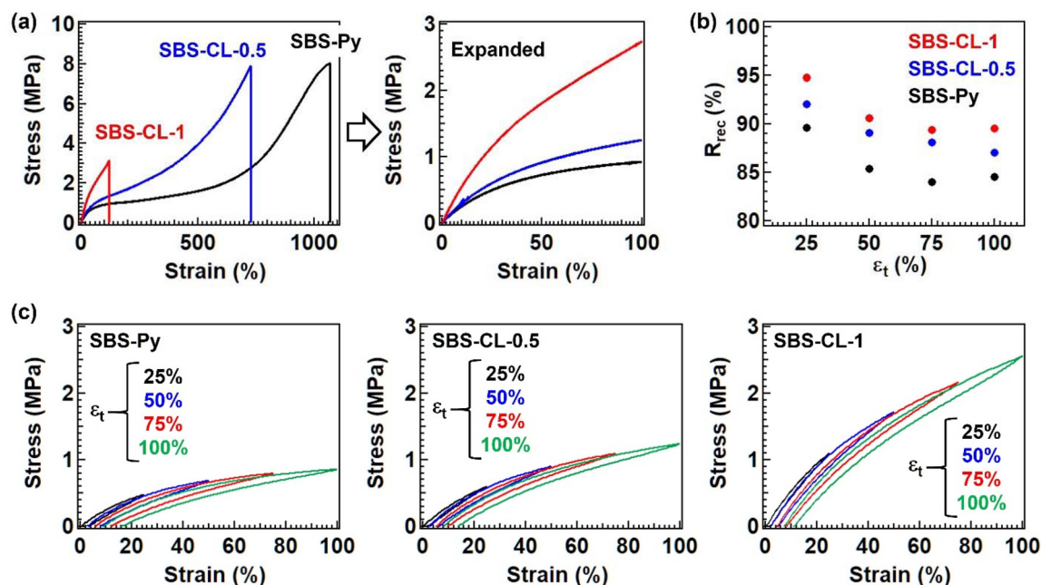
Fig. 6 (a) Stress-strain curves and (b) plots of the recovery ratio ( R_{\text{rec}} ) at different target strains ( \epsilon_t ) for SBS-Py, SBS-CL-0.5, and SBS-CL-1. (c) Raw data of the cyclic stress-strain curves.
