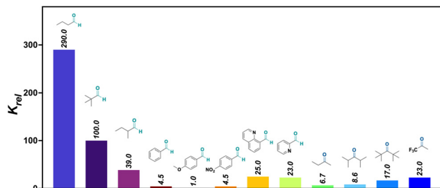
Fig. 14 Relative formation rates ( K_{rel} ) of hydrazones from a selected set of aldehydes and ketones at pH 7. 127 The relative reaction rates refer to the hydrazone formation between either aldehyde or ketones and phenylhydrazine [ K_{rel} (4-methoxybenzaldehyde) = 1]. 67
