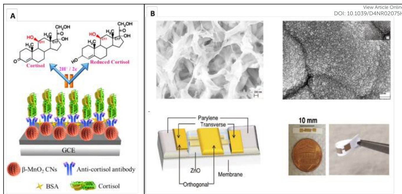
Fig. 8 A) Schematic representation of MnO 2 nanocacti electrochemical biosensor; 128 B) TEM pictures of the polyamide matrix before and after the deposition of ZnO, scheme of the electrochemical biosensor and real-life image of the biosensor. 129
