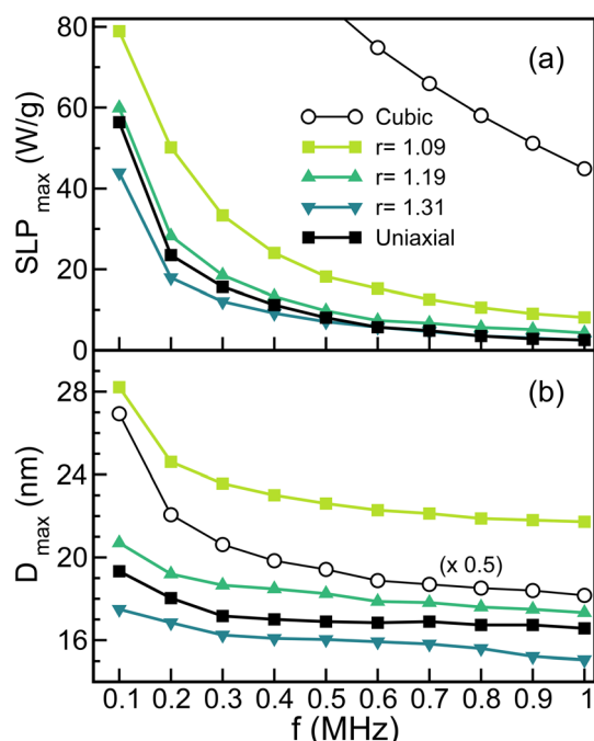
Fig. 8 Frequency dependence of the (a) maximum SLP and (b) the corresponding particle size extracted from the curves in Fig. 7 for different nanoparticle elongation ratios r = 1.09 , 1.19 , and 1.31 (colored symbols) and also for the cases of only uniaxial (black squares) or only cubic contribution (empty circles) with K_{u,c} = 1.1 \times 10^4 \text{ J m}^{-3} . Notice that D_{\max} for the last case has been rescaled by 0.5.
