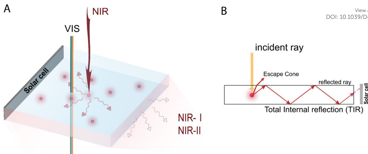
Figure 1. A) Sketch of a transparent LSC, B) working principle of LSCs
