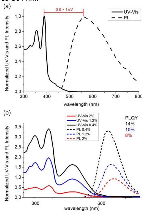
Figure 3. (a) UV-Vis (solid) and PL (dashed) spectra in PMMA matrix of compound 2 . (b) UV-Vis and PL spectra of compound 6 in PMMA matrix at concentrations of 0.4% (black), 1.2% (blue) and 2% (red) respectively. Partially reproduced from 42 and 47. Copyright 2015 and 2022 Wiley.
