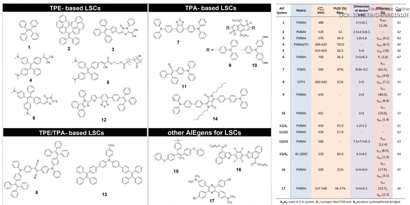
Figure 2. Left: Chemical structures for AIE luminophores used in LSCs; right: main photophysical parameters and performance for AIEgens used in LSCs reported in literature. Efficiency values are reported as: \eta_{int} = (no. of edge-emitted photons)/(no. of total absorbed photons); \eta_{ext} = \eta_{edge} = (no. of edge-emitted photons)/(no. of total incident photons); \eta_{opt} = I_{(SC,LSC)}/I_{(SC,PV)}G , where I_{(SC,LSC)} is the short circuit current generated by a PV cell edge-coupled to the top-illuminated LSC, I_{(SC,PV)} is the short circuit current of the same PV cell under direct illumination from the same light source, and G = A_{top}/A_{edge} , with A_{top} = LSC top surface area, and A_{edge} = LSC edge surface area; P_r is the power generated by the PV cell edge-coupled to the LSC ( P_{LSC} ) to the power produced by the PV cell ( P_{PV} ) under direct exposure (in both cases, illumination was by an AM1.5G solar simulator under one Sun
