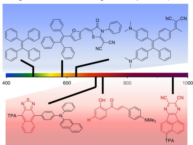
Figure 5. Examples of chemical structures of AIEgens with emissive properties in different spectral regions (TPA = triphenylamine). Blue background: UV-vis responsive AIEgens proposed in the LSC literature ( 41,43,45 from left to right); red background: chemical platforms to be potentially employed for DR/NIR-responsive LSCs ( 57 58 59 from left to right).
