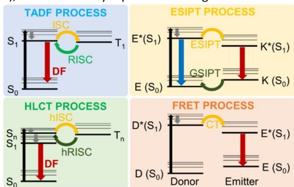
Figure 6. Schematic representation of the TADF, HLCT, ESIPT and FRET photophysical processes.
