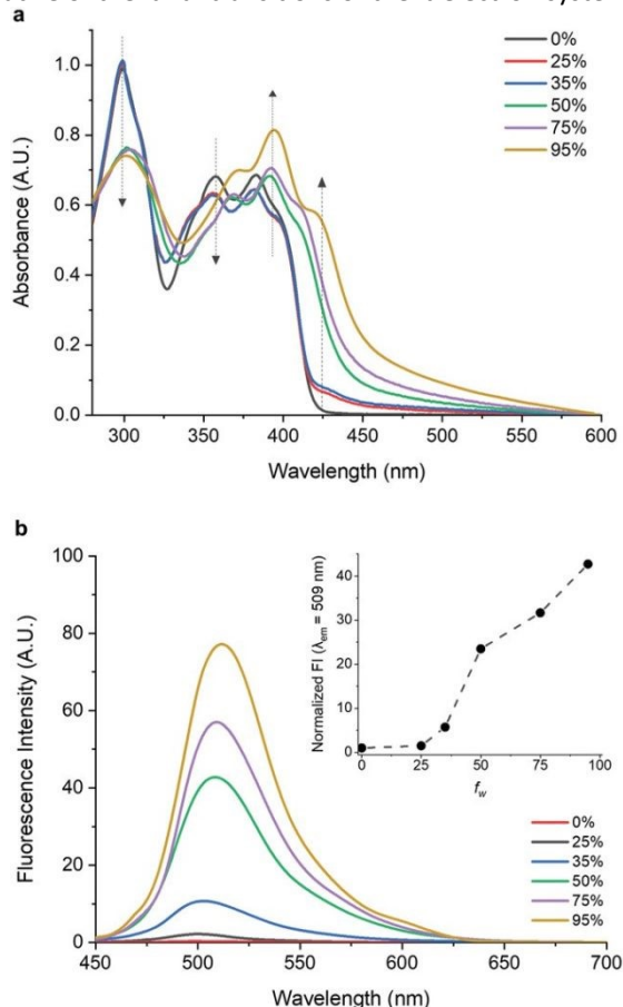
Figure 4. (a) UV-vis spectra of dilute solutions of 16 in THF-H 2 O mixtures with different volume fractions of water ( f_w ). (b) PL spectra of 16 in THF-H 2 O mixtures at different f_w values. The inset shows the normalized PL intensity at as f_w changes. Partially reproduced with permission from ref. 55. Copyright 2021 Wiley
