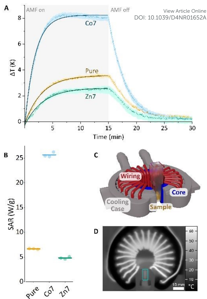
Figure 6 – (A) Hyperthermia measurement. Temperature kinetics of pure, Co7, and Zn7 MFT sample (each 35 \mu\text{M} ) during exposure to the alternating magnetic field (45 mT, 93.75 kHz). Each curve is an average of three runs. The absolute temperature change \Delta T refers to the temperature increase above the temperature of pure buffer solution. All MFT and buffer solution samples measured in an identical manner. (B) Specific Absorption Rate (W/g) of each run (coloured dot) and average value (coloured line). (C) Custom-made hyperthermia setup. (D) Selected thermal image of that was taken during hyperthermia measurement, with the sample (blue box) in the centre of the magnet gap.
