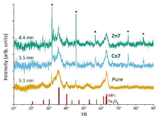
Figure 4 – X-ray diffraction of Magnetoferriin (Pure) and doped (Co7, Zn7) samples using Cu-K \alpha radiation. Runs I-III were pooled. Sharp peaks indicated by asterisks originate from residual NaCl after drying. Crystallite sizes from Scherrer analysis are given on the left. Sticks in black and red indicate the angles and intensities for Fe _3 O _4 and MFT powder samples, respectively. Diffraction patterns are shifted vertically for better visibility.
