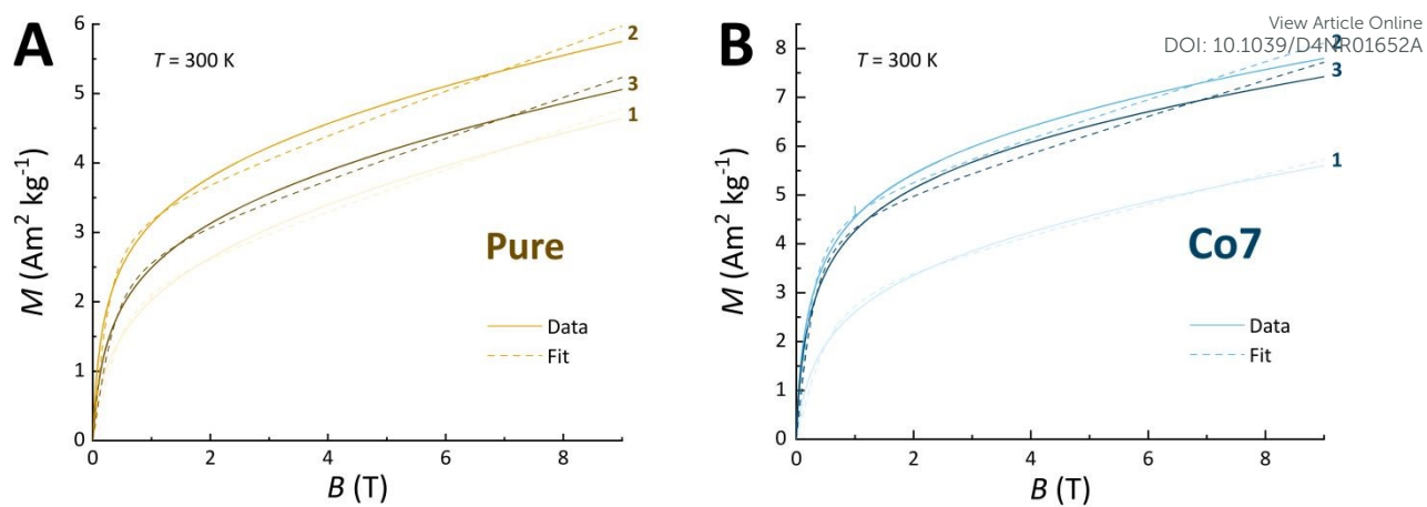
Figure S3 - Langevin Fits. Measured magnetisation and Langevin fits of pure MfT and Co7 samples. Here, we use the Langevin function and an additional linear slope accounts for add-on contributions of salts, organics and possible antiferromagnetic contributions in the samples.
