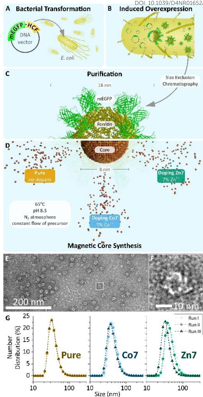
Figure 1 – (A–D) Schematic overview of MFT production. Apoferritin (yellow, PDB code: 1FHA), genetically fused to mEGFP (green, PDB code: 2Y0G, created with Avogadro v. 1.2.0 90 and blender v.2.93.2, Blender Foundation, Amsterdam, Netherlands), is expressed in transformed E. coli and then purified via size exclusion chromatography. Empty cages are filled with their respective metal oxide core (brown) during magnetic core synthesis. (C and D) Scheme of semi-synthetic MFT cage. The three different cores used in this study are indicated. (E) Transmission electron microscopy image of pure MFT's protein shell, stained with 2 % uranyl acetate. (F) Magnified section of E displaying one single ferritin cage. (G) Hydrodynamic radii obtained via dynamic light scattering for MFT with three differently doped cores over three independent synthesis runs.
