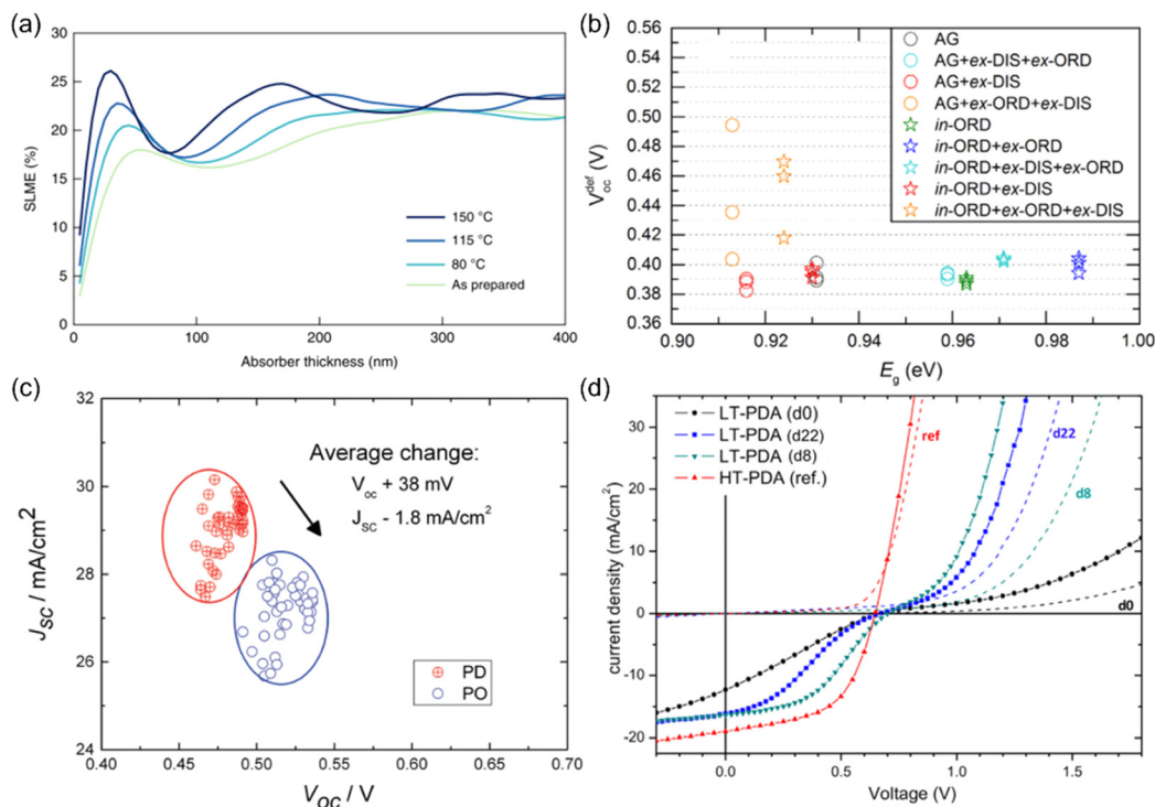
Fig. 3 Impact of cation disorder on photovoltaic performance. (a) The spectroscopic limited maximum efficiencies (SLMEs) of \text{AgBiS}_2 NC films as a function of thickness and annealing temperature, which changes the degree of cation disorder. Reprinted with permission from ref. 31. Copyright 2022, Springer Nature. (b) Open-circuit voltage deficit ( V_{\text{OC}}^{\text{def}} ) of solar cells fabricated based on \text{Cu}_2\text{ZnSnSe}_4 with different degree of cation disorder and hence different bandgaps E_g . Reprinted with permission from ref. 53. Copyright 2016, Elsevier. (c) A set of short-circuit current density ( J_{\text{SC}} )-open-circuit voltage ( V_{\text{OC}} ) data points acquired from the same batch of \text{Cu}_2\text{ZnSnSe}_4 solar cells. PD and PO refer to highly cation disordered and relatively cation ordered \text{Cu}_2\text{ZnSnSe}_4 , respectively. Reprinted with permission from ref. 42. Copyright 2016, John Wiley and Sons. (d) Current density–voltage curves of \text{Cu}_2\text{ZnSnS}_4 devices with different degrees of cation disorder. LT-PDA and HT-PDA refer to the post deposition annealing at low (160 °C) and high temperatures (300 °C), respectively. LT-PDA could lead to a higher degree of cation order, while HT-PDA tended to lower the degree of cation order. “dx” in the brackets refers to the x^{\text{th}} day after device fabrication. Reprinted with permission from ref. 41. Copyright 2017, John Wiley and Sons.
