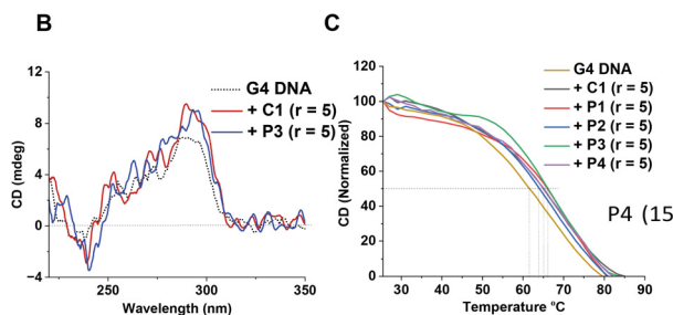
Fig. 2 (A) Chemical structure of NA-TACs ( P1–P4 ) and their control compound C1 . (B) CD spectra of 3 \mu\text{M} Hum 21-mer G4 DNA alone, with compound C1 and with P3 (15 \mu\text{M} ) in 10 mM Tris-HCl (pH 7.4) containing 0.1 M KCl and 0.1 mM EDTA. (C) CD melting profiles of the pre-formed Hum 21-mer G4 DNA alone, and G-quadruplex DNA incubated with ligands C1 , P1 , P2 , P3 , and P4 (15 \mu\text{M} ) in 10 mM Tris-HCl (pH 7.4) containing 0.1 M KCl and 0.1 mM EDTA.
