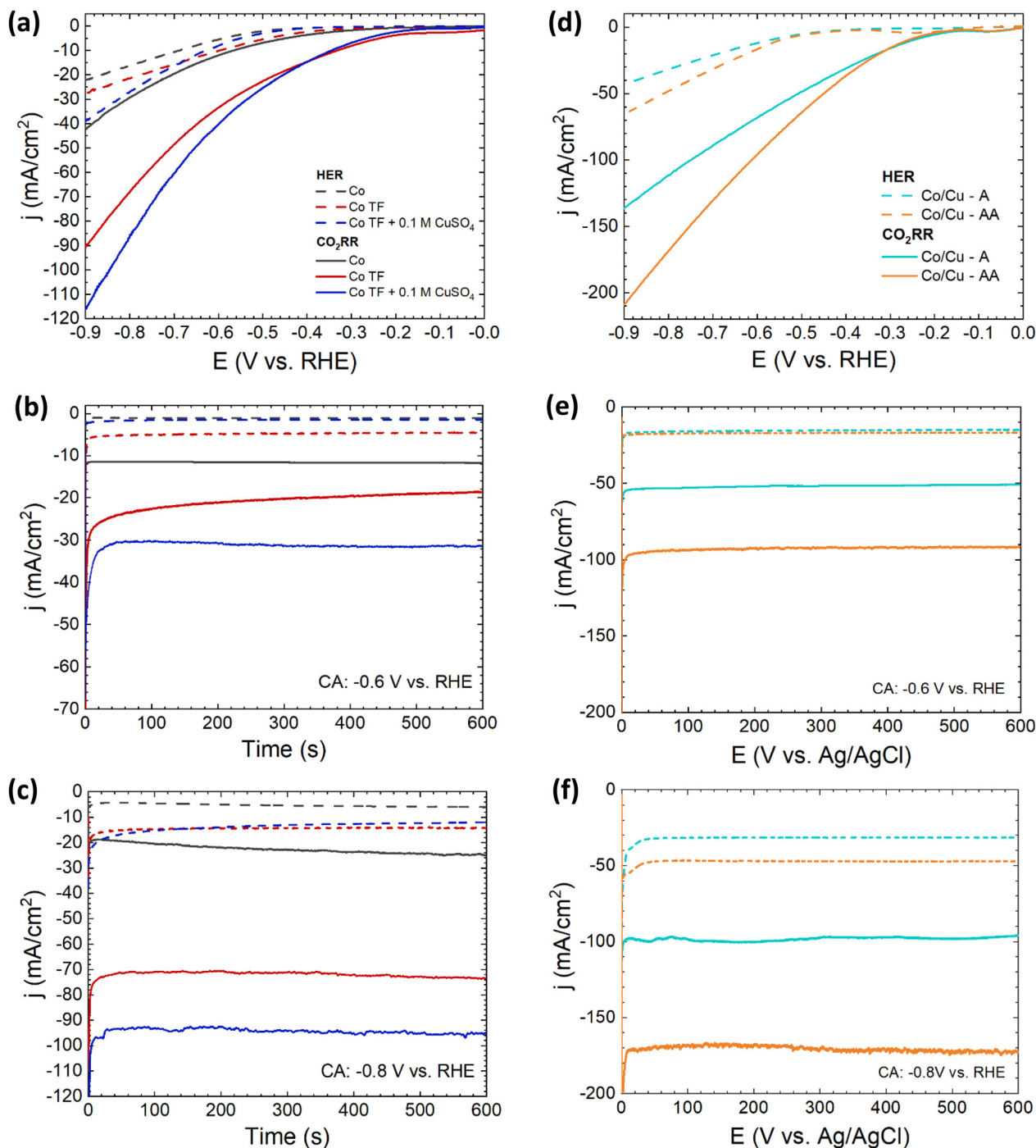
Fig. 3 (a & d) LSVs of (a) the Co substrate (black), Co TF (red), CoTF + 50 \mu L of 0.1 M \text{CuSO}_4 (blue), Co/Cu-A (turquoise), and Co/Cu-AA (orange) electrodes recorded at 20 \text{ mV s}^{-1} scan rate. Dashed lines represent HER experiments conducted in Ar-saturated 0.5 M \text{K}_2\text{SO}_4 (adjusted pH 8.0) and solid lines represent \text{CO}_2\text{RR} experiments conducted in \text{CO}_2 -saturated 1 M \text{KOH} (pH 8.0); (b & e) corresponding CA curves of the electrodes measured at -0.6 \text{ V vs. RHE} for 600 s; and (c & f) corresponding CA curves of the electrodes measured at -0.8 \text{ V vs. RHE} for 600 s.
